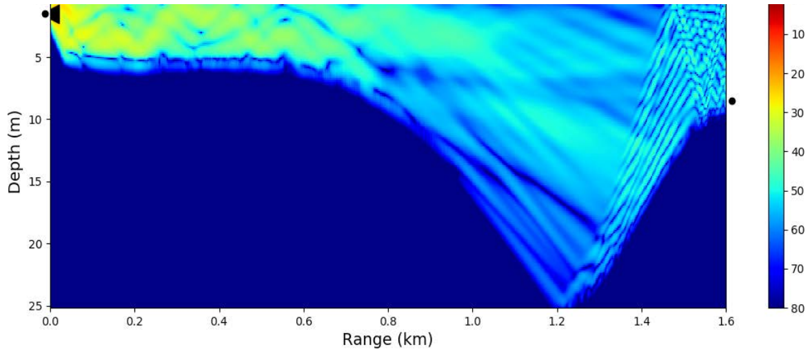
Fig.4: Transmission loss simulation at frequency 8360Hz with the environmental characteristics of the site of BIOCUM'19 sea trial using isovelocity sound speed profile.
