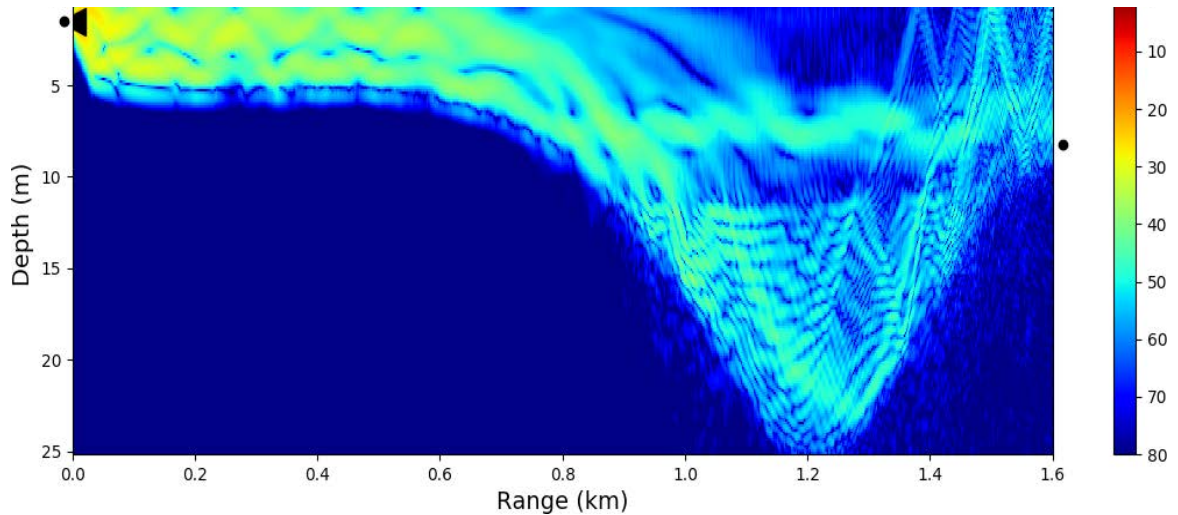
Fig.5: Transmission loss simulation at frequency 8360Hz with the environmental characteristics of the site of BIOCUM'19 sea trial using the sound speed profile captured on January 15, with severe downward refraction due to upwelling.
