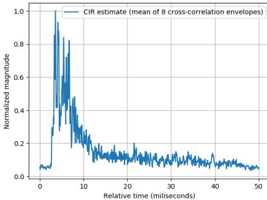
Fig.2: Channel Impulse Response (CIR) normalized estimate for the source-receiver transect of the BIOCOT'19 sea trial at time 10h20m on January 18, 2019.
